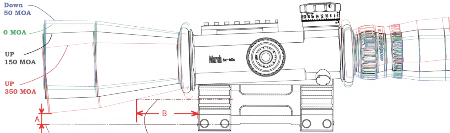
External dimensions when mounting with standard mount (mm)
